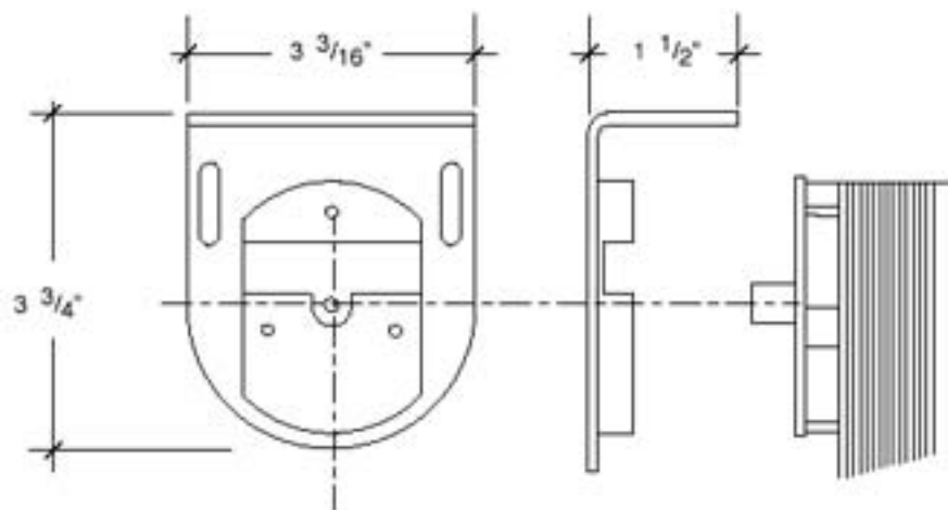
Idle End Bracket
